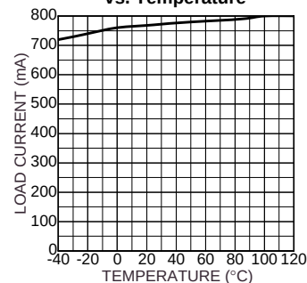
S/C Current vs. Temperature
