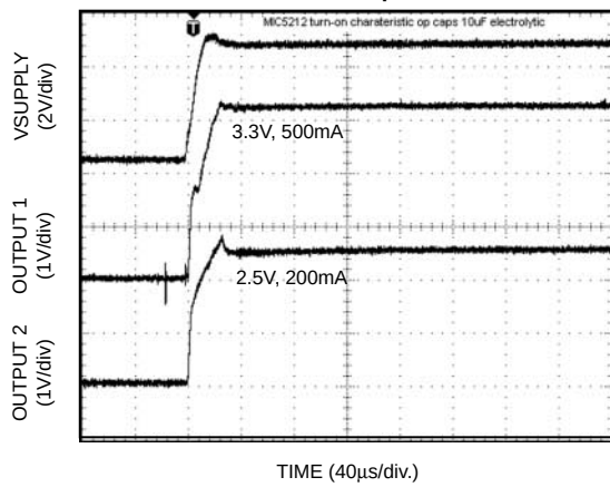
Turn-On Response
